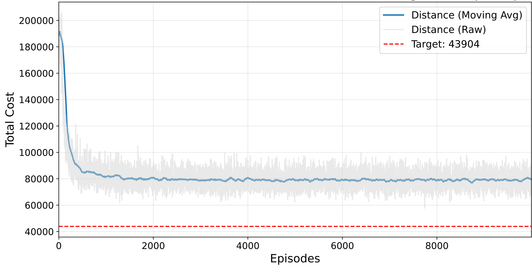
Final GAUSSIAN PROCESS Masked AutoRL-SOP Training - kro124p.3.sop
